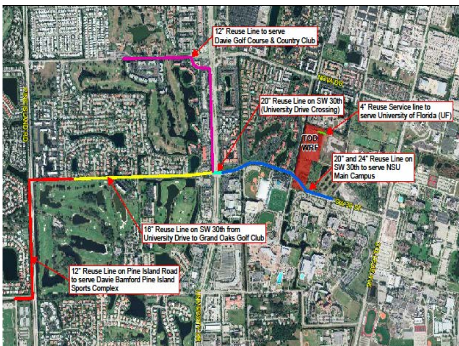
Map. Town of Davie Utilities Water Reclamation Facility (WRF) – Reclaimed Water availability layout
